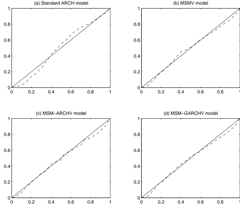
Figure 3: Cumulative distribution functions corresponding to the probability integral transforms associated with the standard ARCH model, the MSMV model, the MSM-ARCHV specification and the MSM-GARCHV model. For each model the dashed line represents the effective cumulative distribution function, whereas the solid line denotes the theoretical cumulative distribution function under the assumption that the sequence of probability integral transforms is iid U(0, 1) .
