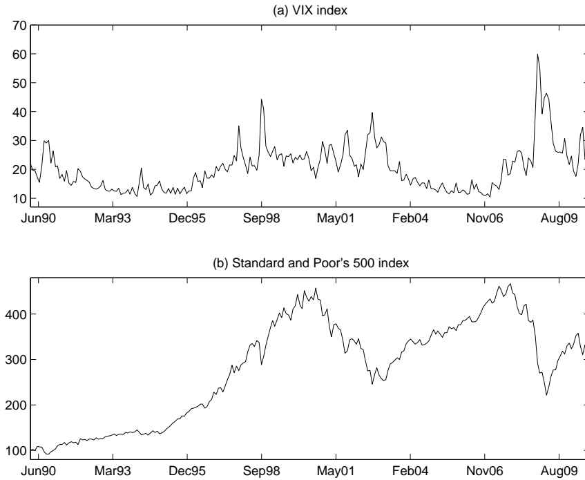
Figure 1: Monthly evolution of the VIX index (panel a) and the Standard and Poor's 500 index (panel b) during the period February 1990 to September 2010. The panel b captures the month-end prices of the Standard and Poor's 500 index, obtained from Bloomberg, as a percentage of the month-end value corresponding to February 1990. The data corresponding to the VIX index are available at www.cboe.com/micro/vix/historical.aspx .
